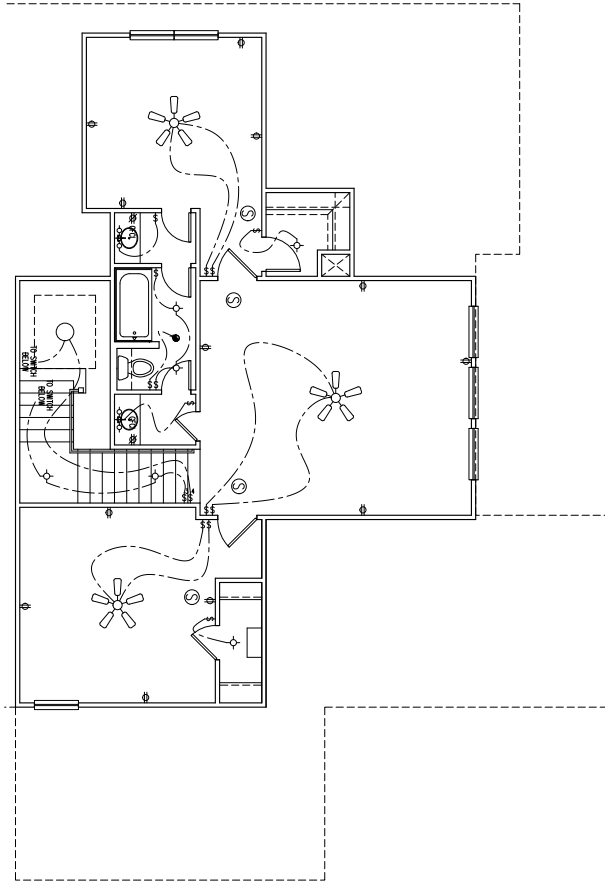
2 SECOND FLOOR ELEC. PLAN SCALE: 1/4" = 1'-0"
