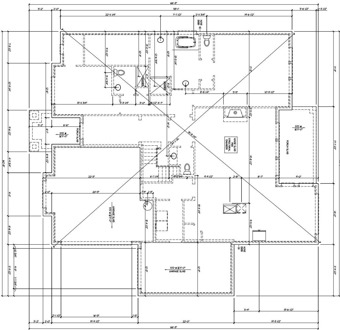
1 FOUNDATION DIMENSION CONTROL SCALE: 1/8" = 1'-0"
