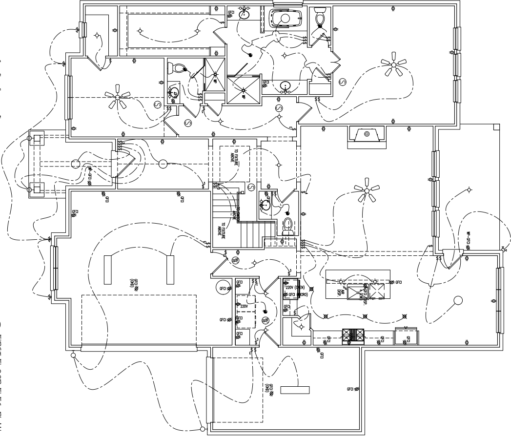
1 FIRST FLOOR ELEC. PLAN SCALE: 1/4" = 1'-0"
