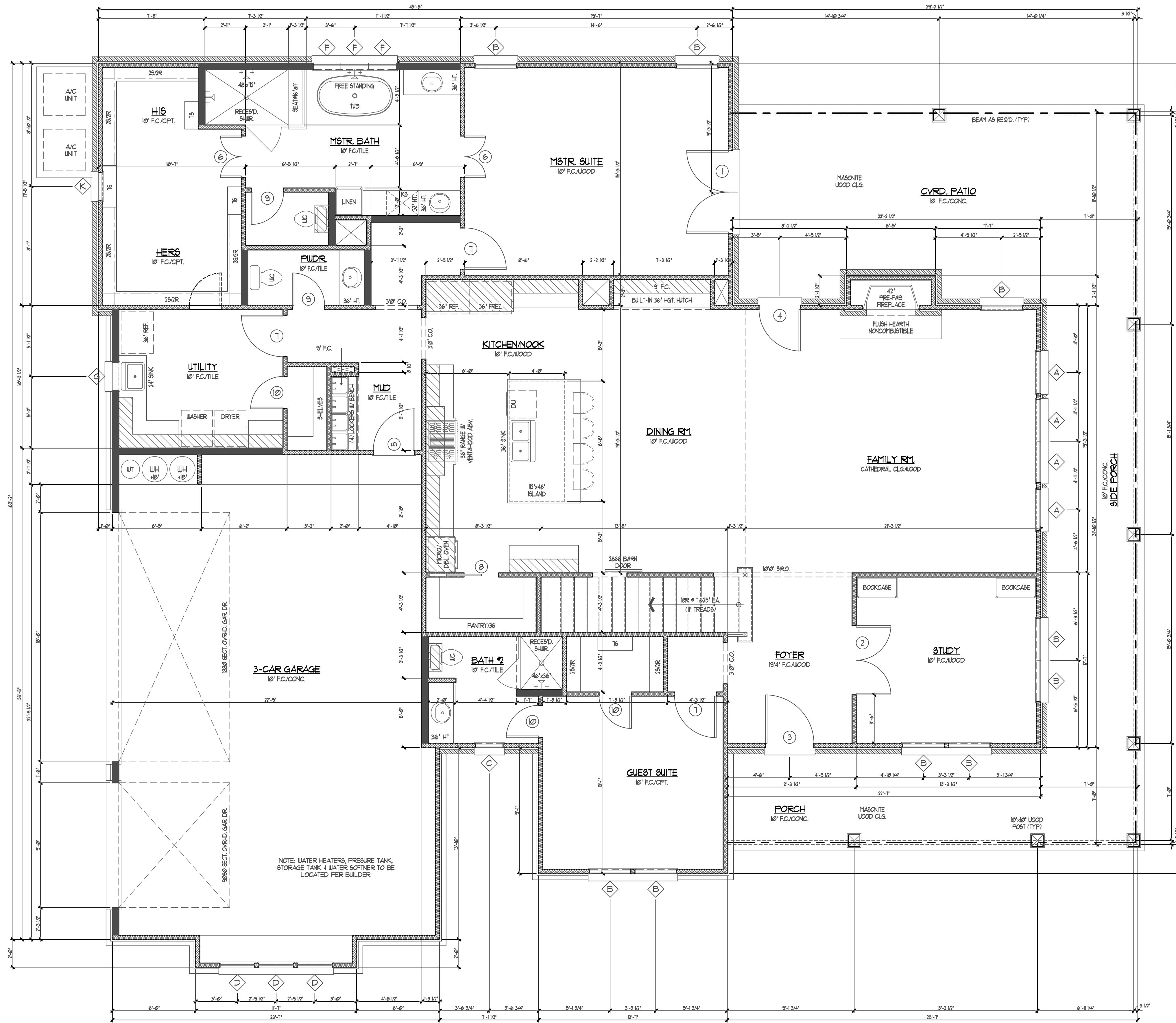
1 GROUND LEVEL FLOOR PLAN SCALE: 1/4" = 1'-0" PLAN NORTH
