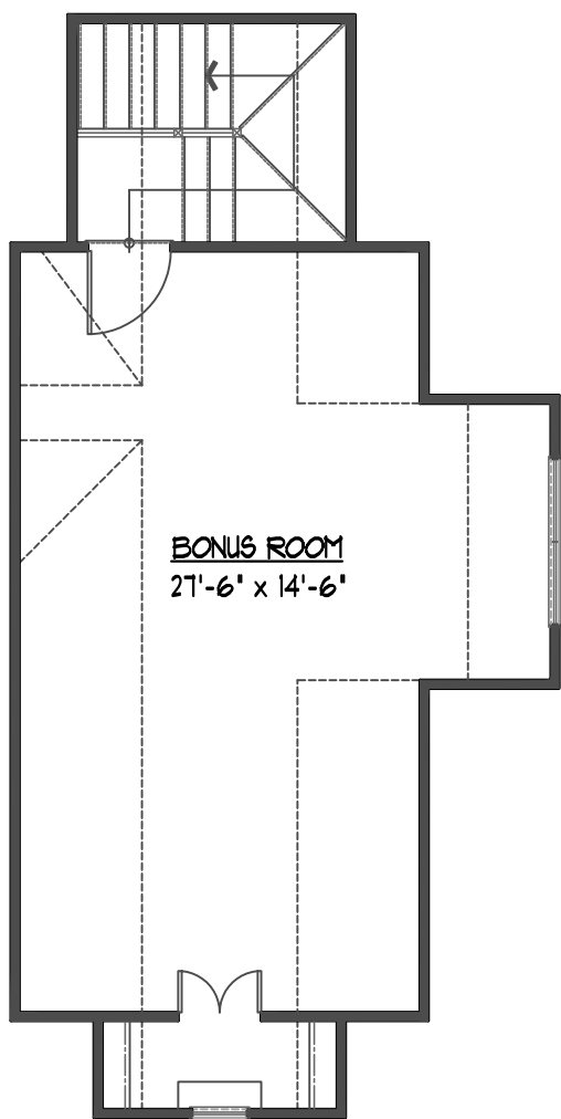
OPTIONAL BONUS ROOM (ADD 505 SF)
